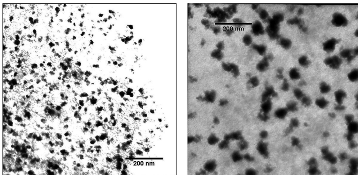
Figure 1. TEM images of the fresh catalyst ( left ) and the reused catalyst ( right ) at the same magnification.
